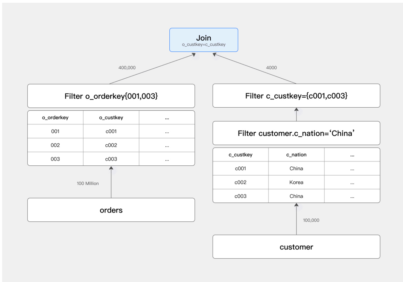
join-runtime-filter-2
