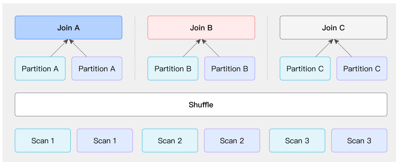
Partition Shuffle Join
